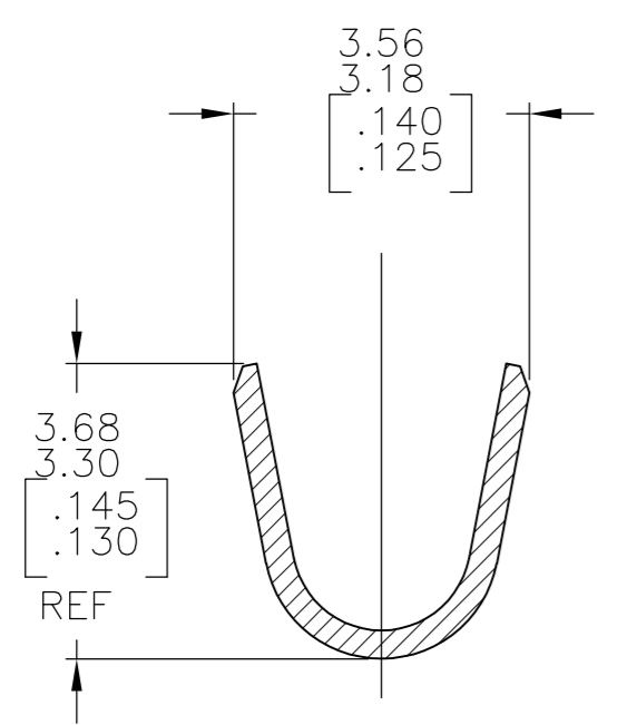
SECTION B-B SCALE 10:1
